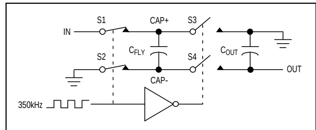
Figure 2. Charging C_{FLY}
